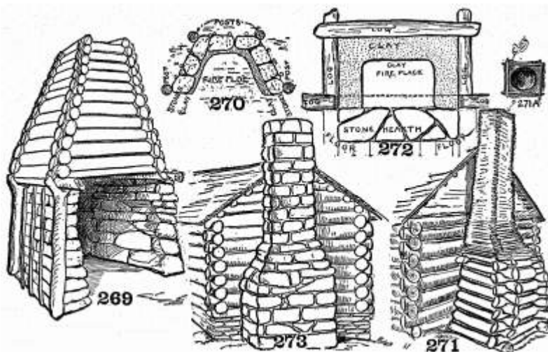
Detail for fireplaces and flues.
