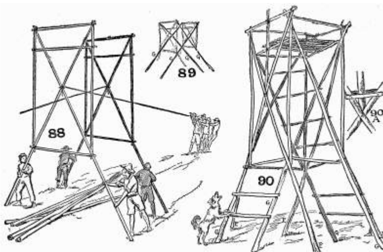
Details of scout signal-tower or game lookout.
